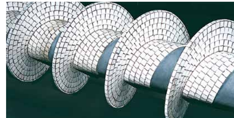
In addition to KALMETALL and KALCAST linings, conveyor screws may also be effectively protected with KALOCER high alumina ceramics. Screw conveyors can have diameters up to 2.000 mm.
