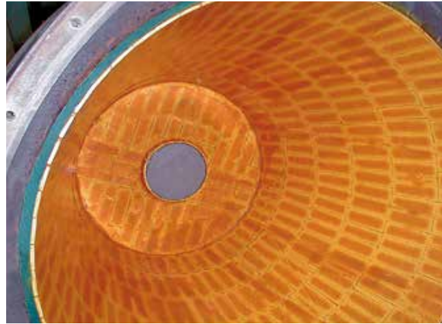
Silo hopper fitted with 25 mm thick KALOCER lining. Due to high requirements on cohesiveness and impact resistance the attachment is fixed with a high performance adhesive.
