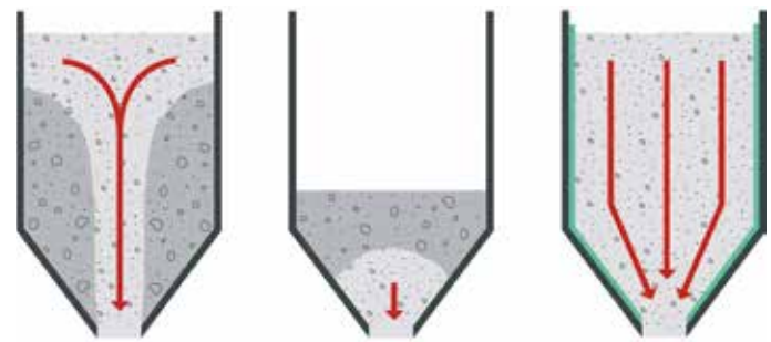
Coatings and core flow
