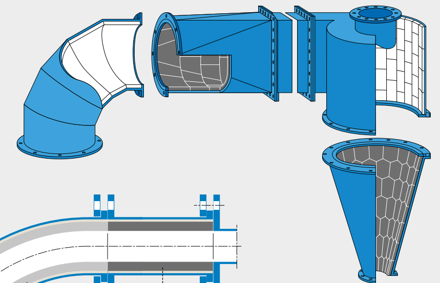
In case of specific applications combinations of Kalenborn wear protection materials may be suitable, e.g. ABRESIST, KALCOR, KALOCER, KALCRET or KALMETALL
