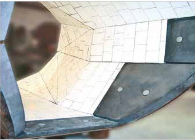
Octagonal hopper subjected to impact stress lined with three-dimensionally cut KALOCER shaped elements as well as KALCAST shapes, each 50 mm thick
