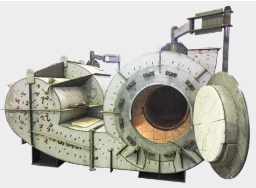
KALCOR protects the convex dryer of a chemical company against abrasion by fine-grained aluminum silicate at high temperature differences
