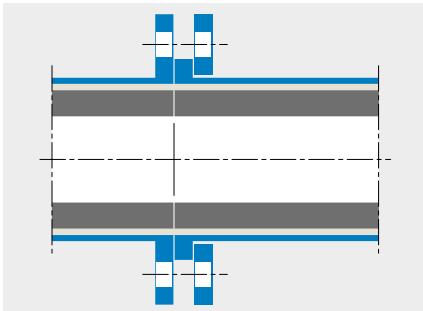
Lined pipes can be connected to each other easily with a fixed collar and a loose turnable flange on one end.
