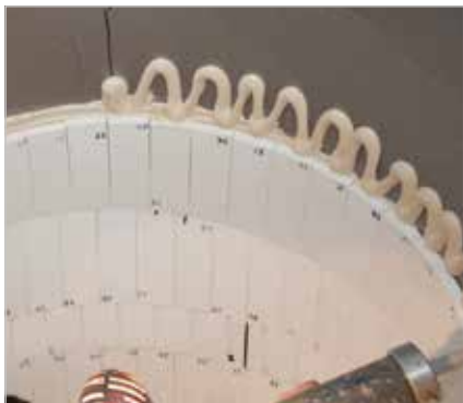
Lining with KALOCER mosaic mats in KALFIX setting compound
