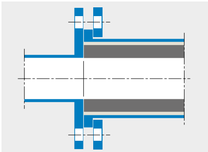
A weld-on counter flange with larger bolt circle diameter on the unlined pipe is a proven solution to connect pipes.
