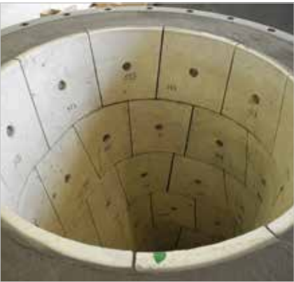
Convex dryer inlet with KALCOR-lined tiles
