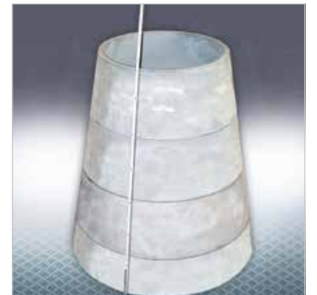
KALSICA lining for a cyclone handling silane dust; major cone diameter 1,200 mm; wall thickness 30 mm
