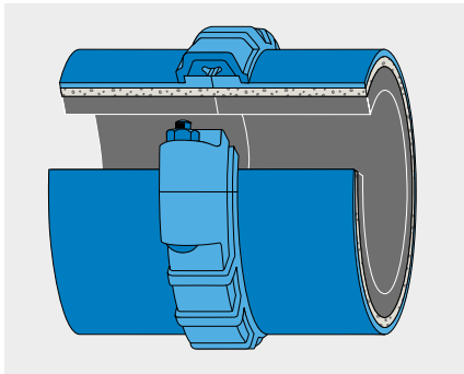
Coupling with axial restraint
