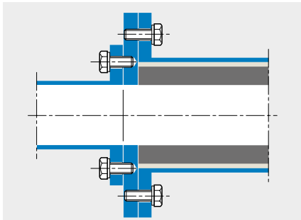
Unlined pipes, pumps or fittings can be connected with a lined pipe using an adapter flange.
